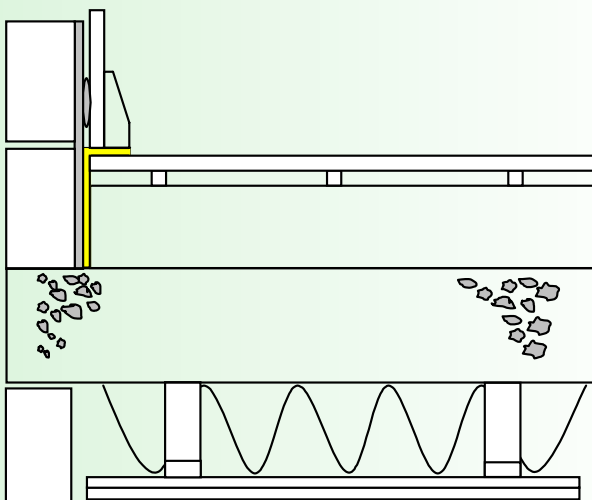
ROBUST DETAIL E-FC-2
